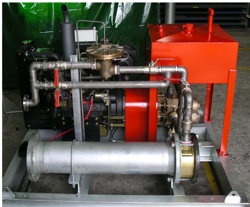
Diesel foam proportioning skid
