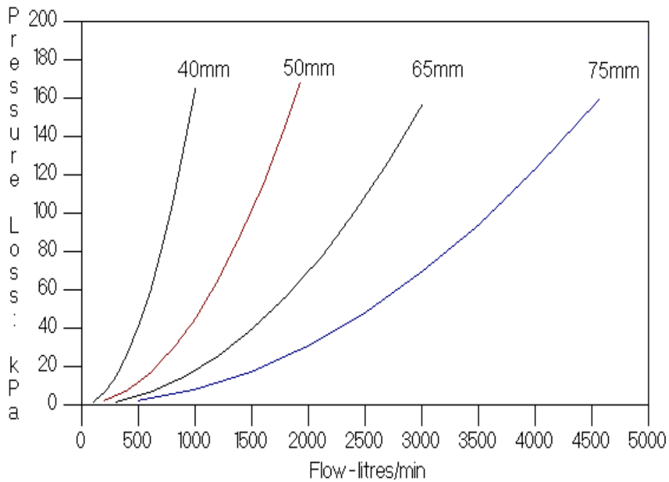
Friction Loss Curve
